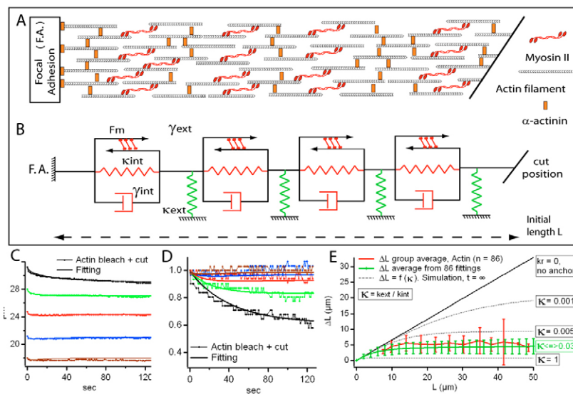
Fig. 2. Viscoelastic model used for data analysis. (A) Schematic view of the internal SF organization with actin, myosin II and the actin crosslinker \alpha -actinin. (B) Representation of the viscoelastic model. In red, the elements of the internal contractile units: spring of stiffness k_{int} , dashpot of viscosity \gamma_{int} and contractile force F_m . In green, the external anchor springs of stiffness k_{ext} . Cytosolic friction is denoted by \gamma_{ext} . FAs and anchoring substrate are considered hard boundaries. Each kymograph was fitted with one set of model parameters. (C) Time course of the bleached stripes positions extracted from Fig. 1E overlapped with the fitted model curves. (D) Normalized stripe width overlapped to the corresponding model curves calculated from C. Colors correspond in C and D. One set of the four model parameters is sufficient to reproduce the non-homogeneous retraction of the whole SF. Fit values for parameters in C and D are (\kappa, \delta, \tau, \tau_e) = (0.067, 0.58 \mu\text{m}, 52 \text{ seconds}, 0.0 \text{ seconds}) . (E) In red, the averaged total retraction \Delta L(L) , reported for Ptk-2 cells in Fig. 1I, shows a very good agreement with the model curve (green), averaged with 86 parameter sets extracted from the actin data (error bars show s.d.). The \Delta L(L) model curve corresponds to an average crosslink ratio \kappa \approx 0.034 (see Appendix 1). For comparison, other \Delta L curves are plotted (dashed lines) with \kappa=1, 0.005, 0.0001 and 0. Note that \kappa=0 would correspond to a free SF, i.e. with no external linkage ( k_{ext}=0 ).
