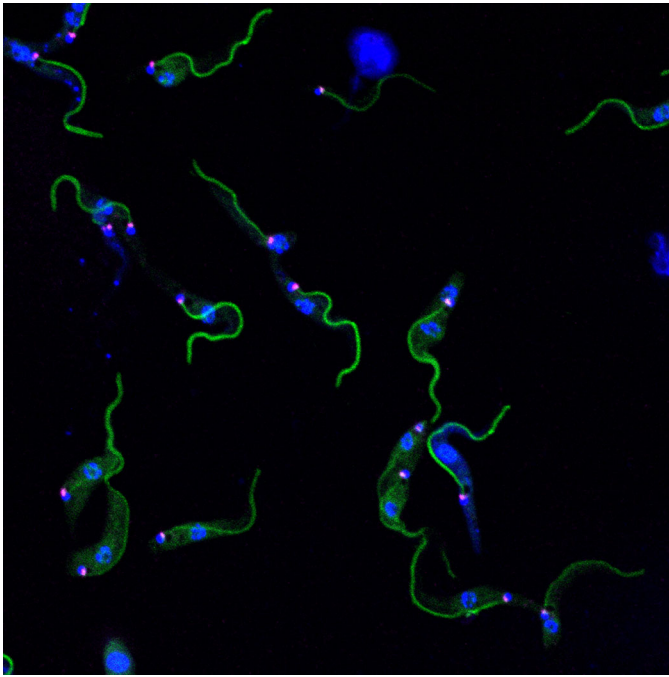
Differential localization of the two Arl3 homologues in T. brucei . TbArl3A (green) is highly enriched along the flagella, while TbArl3C (magenta) is specifically located at the flagellar base. Cells were imaged live, with cell-permeable DAPI to mark the nuclei and kinetoplasts.
