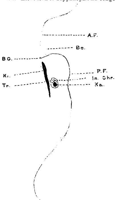
TEXT-FIG. 1.—Active form of Trypanoplasma congeri .
