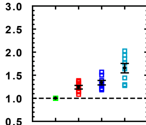
EGFP- \beta -Actin Grid
