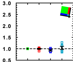
EGFP- \beta -Actin Cross
